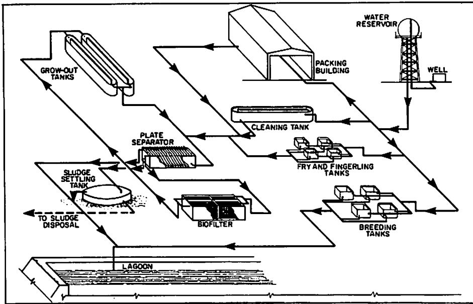
Fig. 1a. Water flow in proposed Kuwait tilapia farm.
