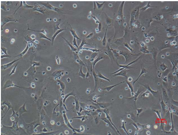
Elongation along with detachment of cells in CFF cell line (derived from Pristolepis fasciatus ) at 6 days post infection following inoculation of filtered tissue homogenate of TiLV infected fish.
