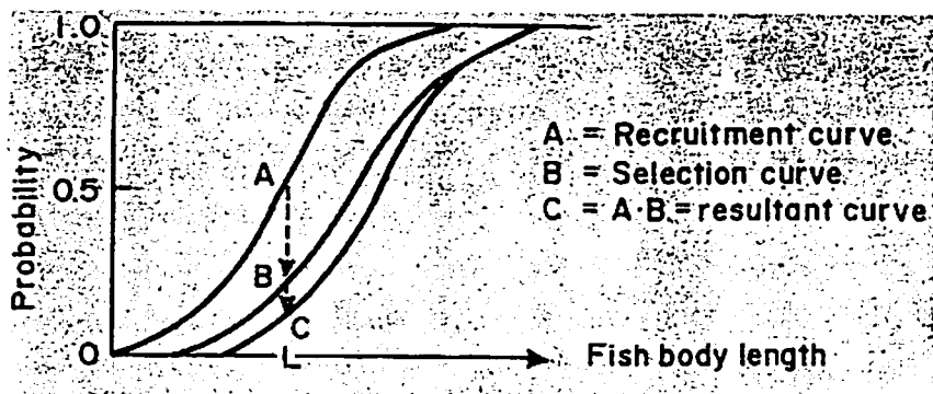
Fig. 1. Definitions and interactions of recruitment, selection and resultant curves. Note that a given C value is simply the product of the A x B values for the corresponding length (L). Fig. 2. Left: growth curve for Peruvian anchoveta, as derived from uncorrected data. Center, upper figure: catch curve, with backward projection as used to estimate probabilities of resultant curve. Center, lower figure: resultant curve, as used to correct original length-frequency data. Right: comparison of initial growth curve (dotted line) with second growth curve (solid line). Note steeper growth curve, due to shift of peaks toward the left (see also text).
