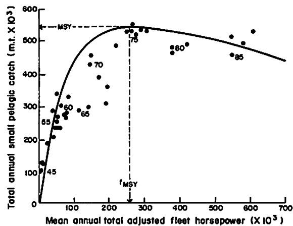
Fig. 1a. Biological surplus production model.
